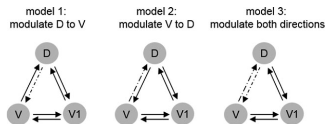
Figure 2. The model space for the DCM analysis. The lines with arrows, either dashed or solid, indicate that there are intrinsic connections between the different ROIs. Dashed lines indicate that a connection is modulated by a specific condition; arrows indicate the direction of that modulation. “V” indicates a ventral tool area, which was either left MTG or left mFG, depending on the analysis that was conducted. “D” indicates a dorsal tool area, which was either left ant IPS or left SPL, again depending on the analysis that was conducted.
